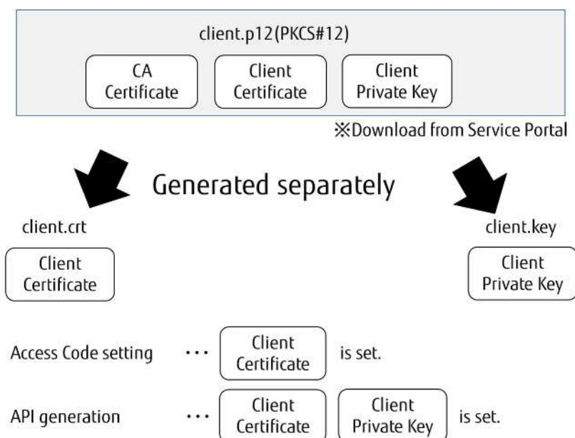
Figure 13 Separating PKCS#12
